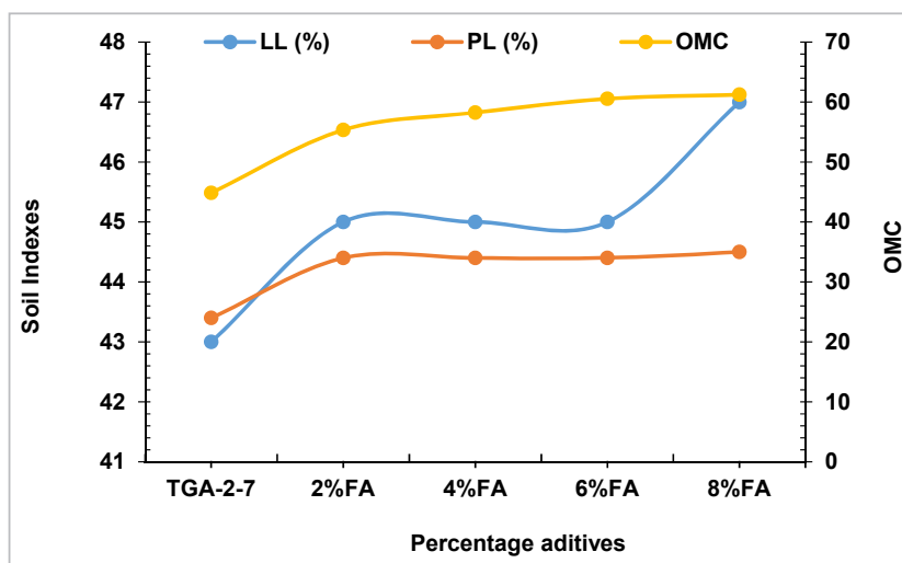
Fig. 2. The impact of FA concentration on the soil PI, PL, and LL
